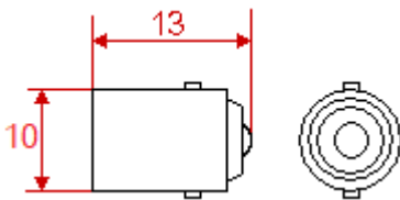
BA10s Sockel-Layout
